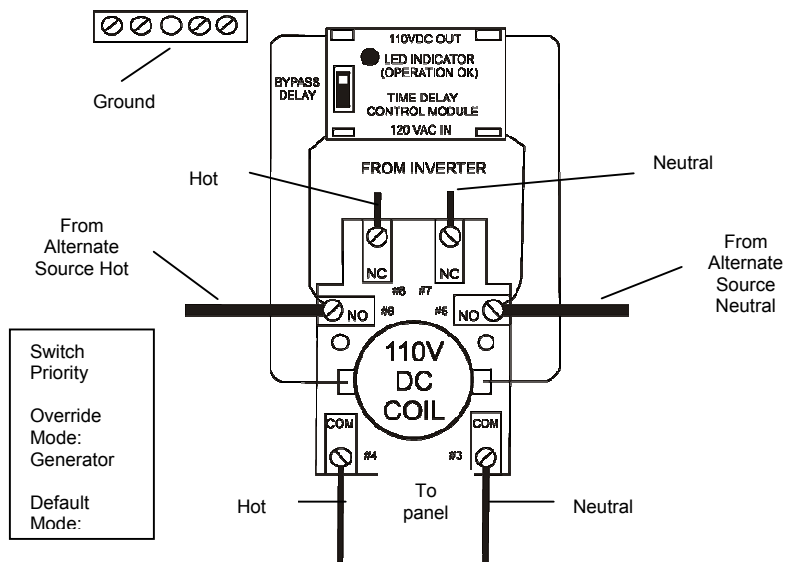
Diagram 2 – Typical Generator inverter / Alternate Source Connection
