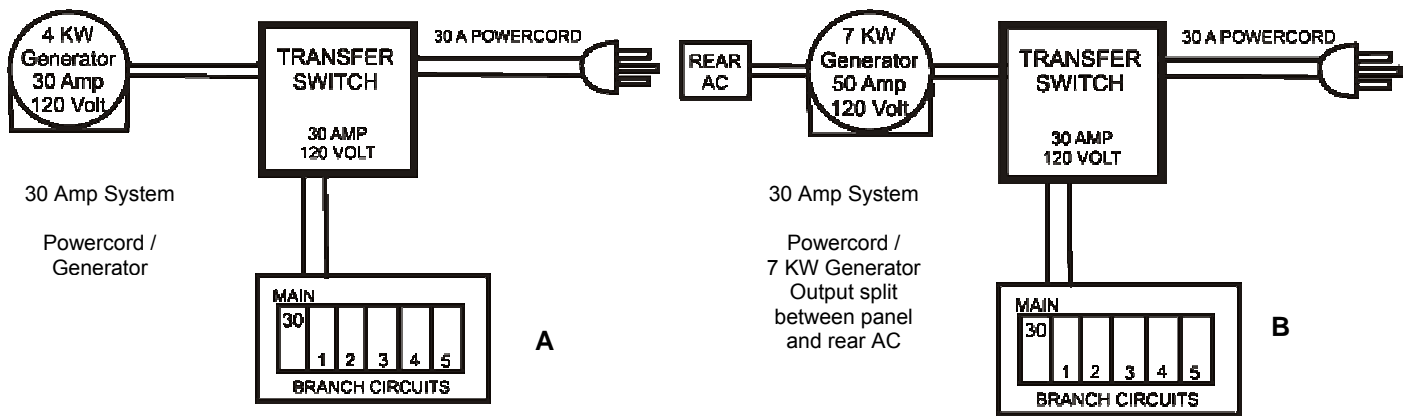
Diagram 1 – Typical Generator Powercord Connection
