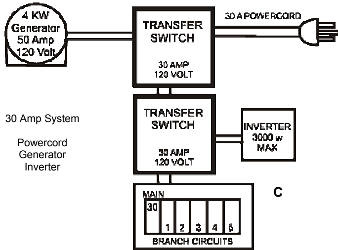
Diagram 2 – Typical Generator inverter / Alternate Source Connection
