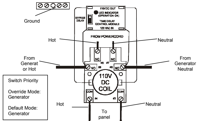
Diagram 1 – Typical Generator Powercord Connection
